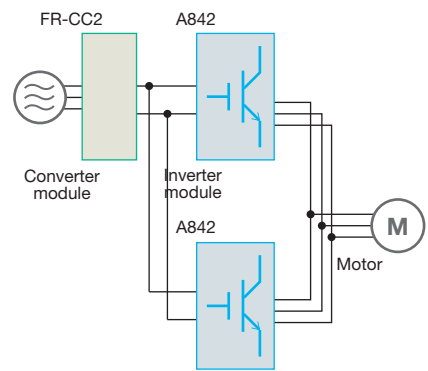
Parallel driving
