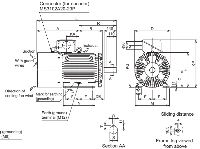
Frame Number 200L, 225S SF-V5RU(H) 30K 37K 45K 55K
