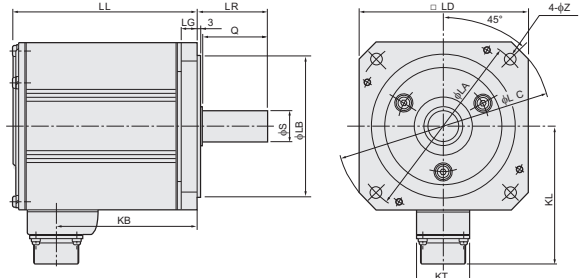
MM-CF□C (Waterproof type)
