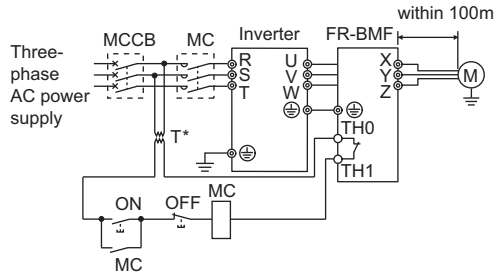
FR-BMF-H7.5K
