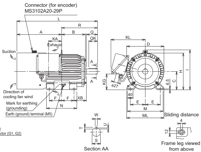
Frame Number 100L, 112M, 132S, 132M SF-V5RU(H) 2K 3K 5K 7K
