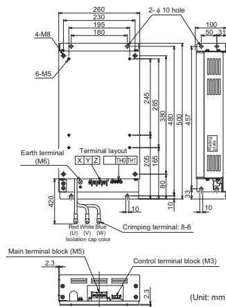
FR-BMF-H15K, H22K
