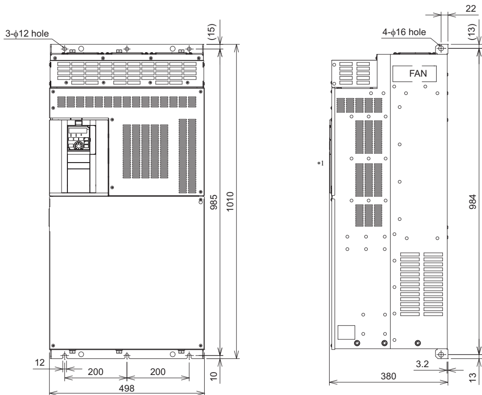
FR-A840-04320(160K), 04810(185K)(GF)
