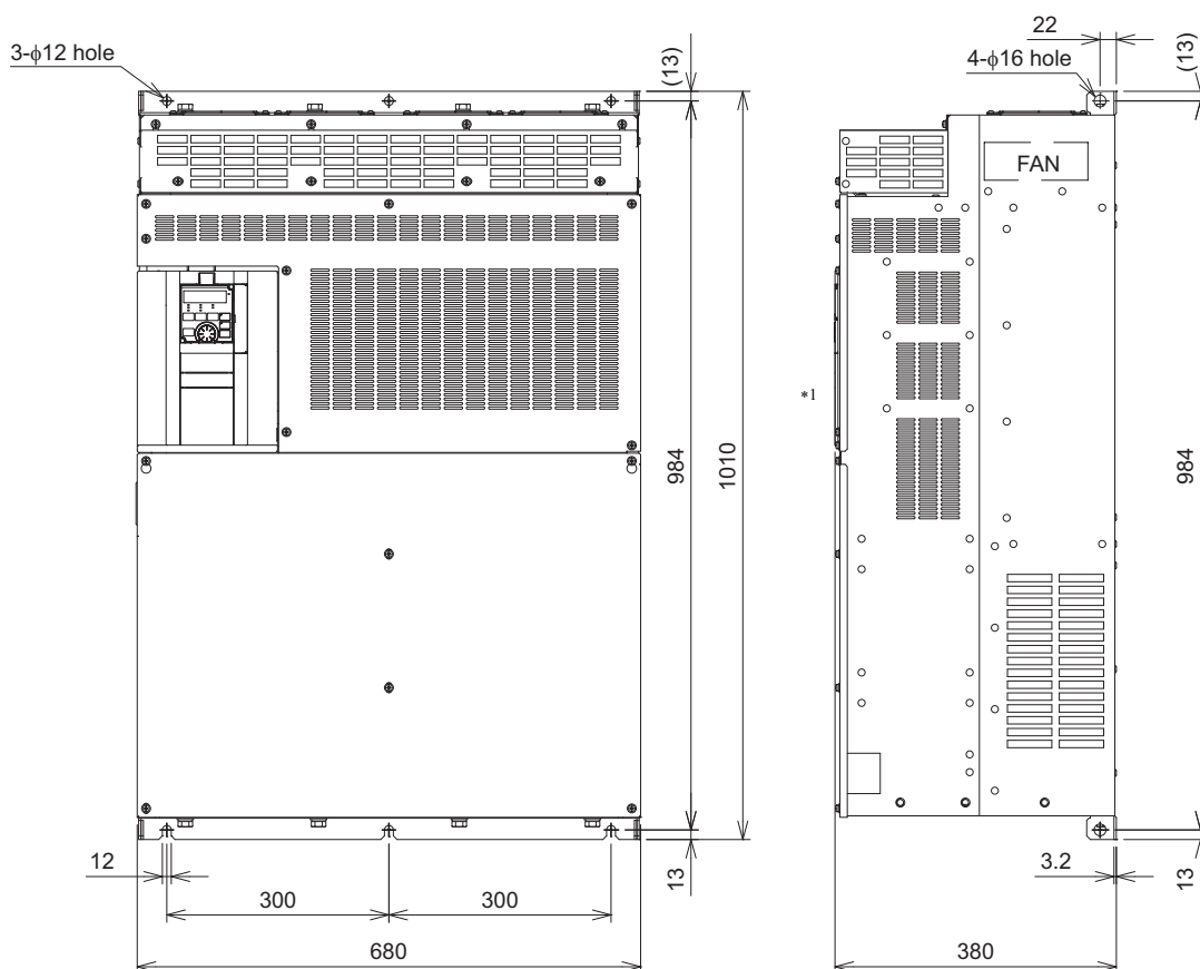
FR-A840-05470(220K), 06100(250K), 06830(280K)(GF)
