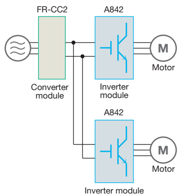
Common bus
